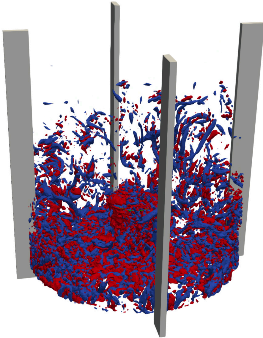
Figure 3: Q-criterion, blue = +40000, red = -40000 (snapshot from simulation video)
