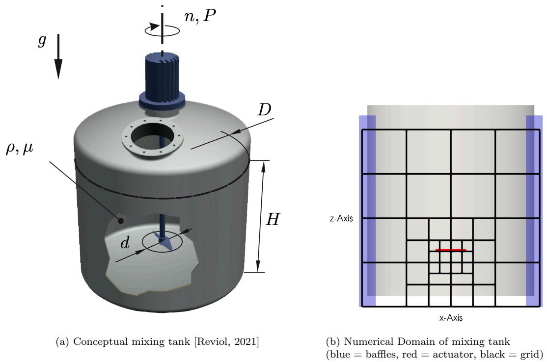
Figure 1: Mixing tank setup with spatial discretisation
