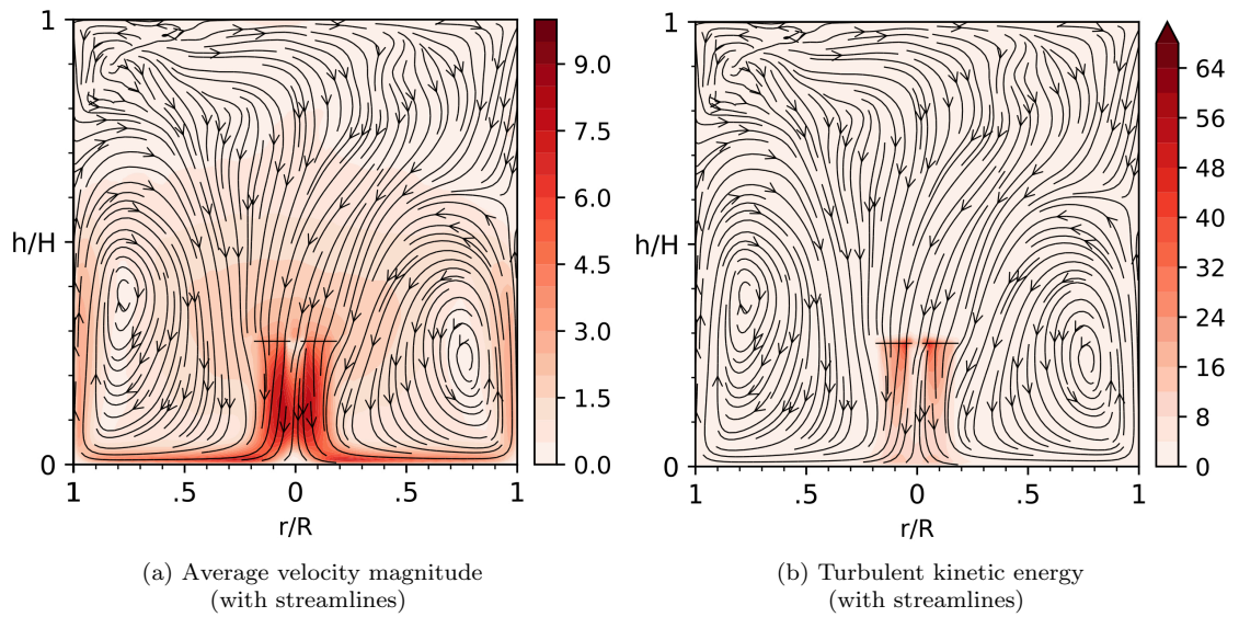
Figure 2: Exemplory simulation results
